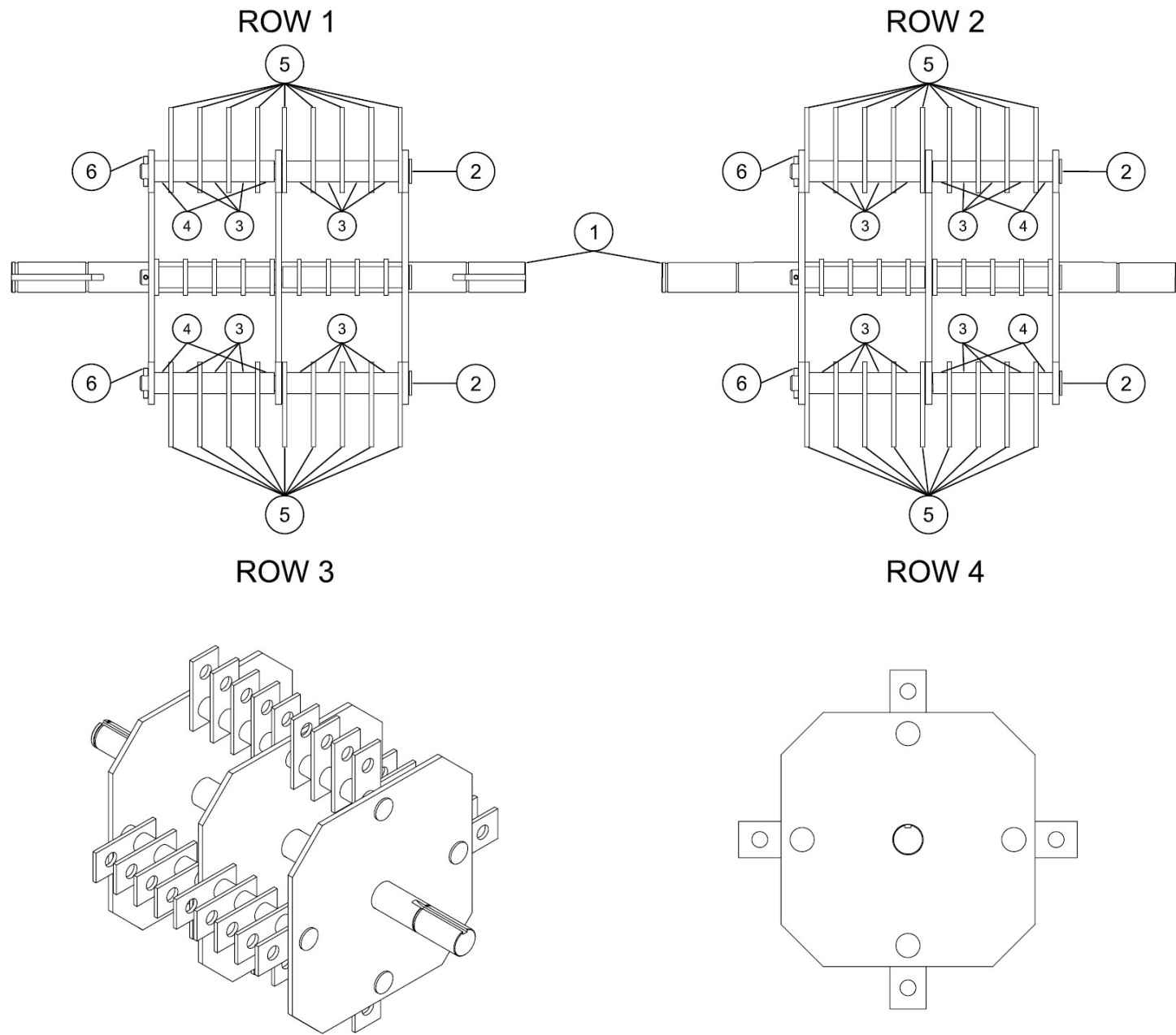
910-0016 ROTOR ASSEMBLY
